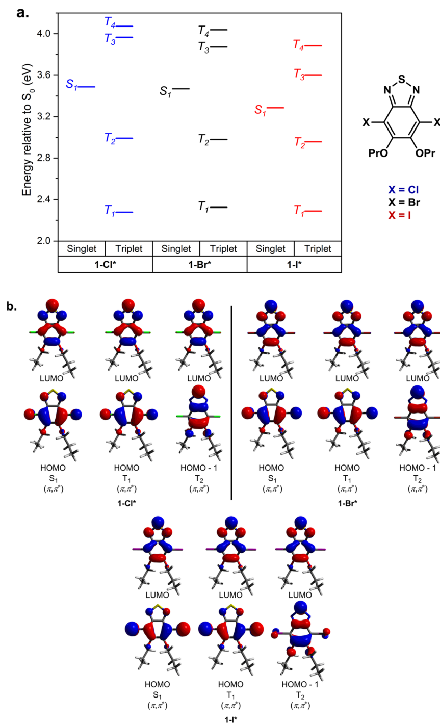
Figure 5. (a) Energy level diagrams for propoxy-functionalized derivatives 1-Cl* , 1-Br* , and 1-I* in the gas phase. (b) Kohn–Sham orbitals representing the electronic configuration descriptions of S_1 , T_1 , and T_2 for each calculated molecule.
