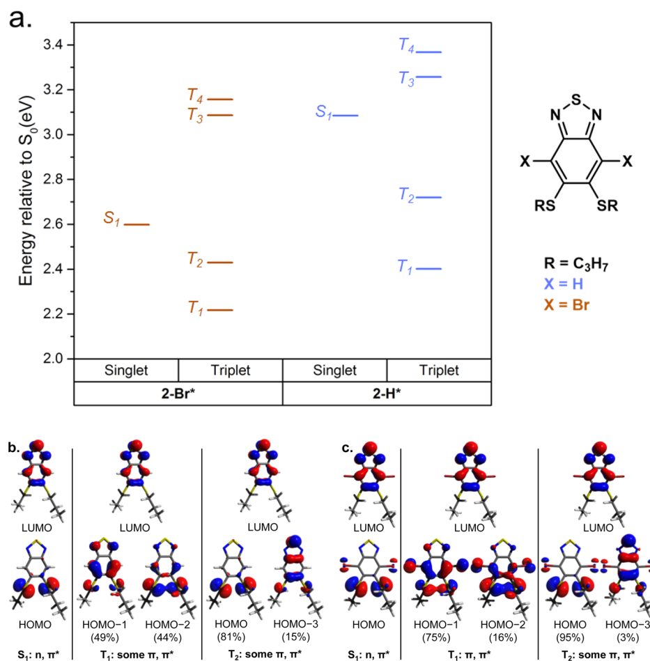
Figure 6. (a) Energy level diagrams for 2-H* and 2-Br* in the gas phase. (b) Kohn–Sham orbitals representing the electronic configuration description of S_1 , T_1 , and T_2 manifolds of 2-H* (b) and 2-Br* (c). Indicated percentages describe the overall character for each displayed transition.
