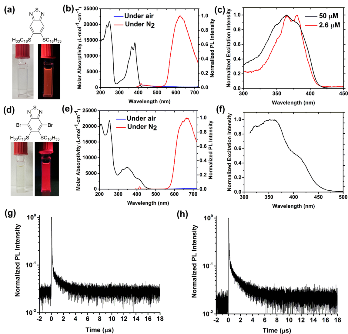
Figure 4. (a) 2-H in cyclohexane with its (b) absorption spectrum and photoluminescence spectra under air and N 2 gas and (c) phosphorescence excitation spectra at 50 μM and 2.6 μM ( \lambda_{em} = 575 nm). (d–f) 2-Br with its corresponding absorption/photoluminescence spectra ( \lambda_{ex} = 370 nm, 50 μM) and phosphorescence excitation spectrum ( \lambda_{em} = 600 nm, 50 μM). (g) Time-dependent photoluminescence decays for 2-H and (h) 2-Br in deoxygenated cyclohexane at 50 μM.
